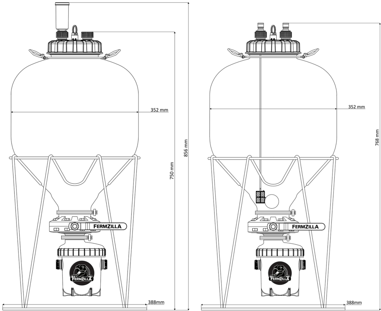
27L FermZilla Tri-Conical Dimensions
