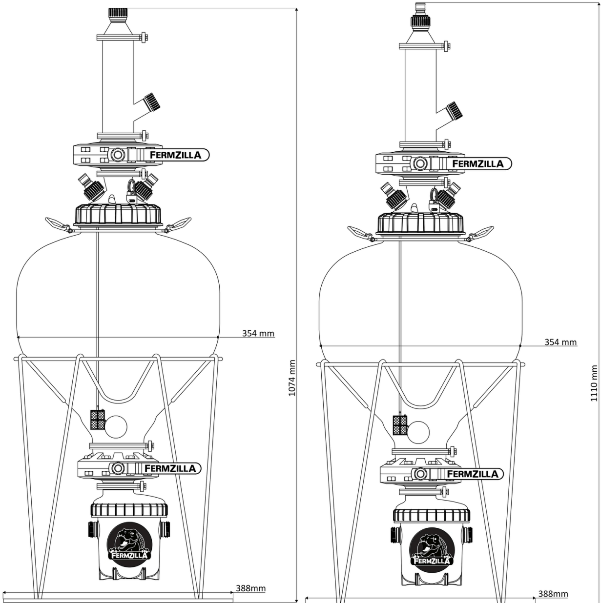
27L FermZilla Tri-Conical Dimensions - Hop Bong + Butterfly Valve
