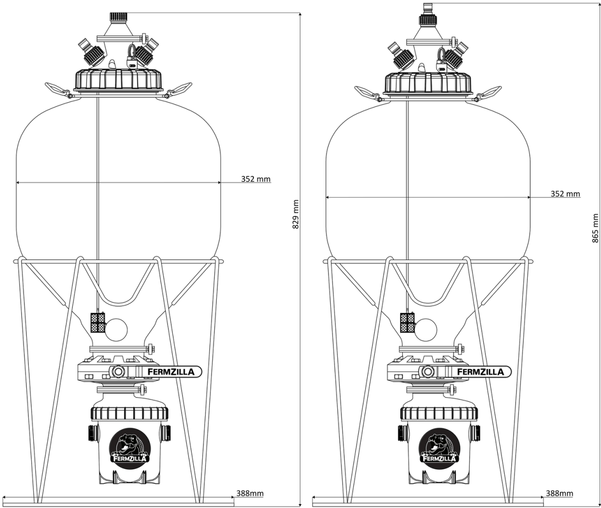
27L FermZilla Tri-Conical Dimensions - Tri Clover Lid
