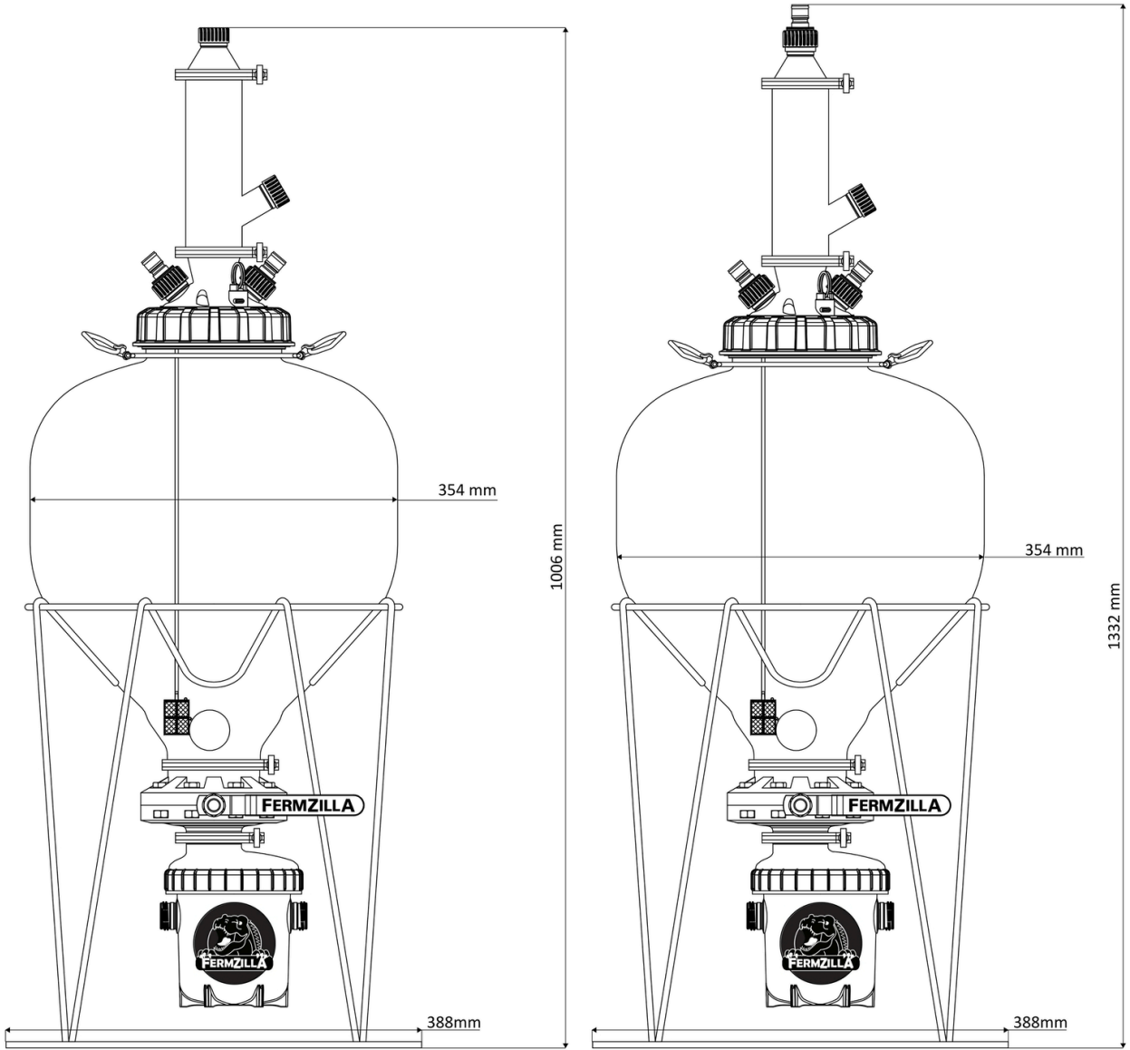
27L FermZilla Tri-Conical Dimensions - Hop Bong
